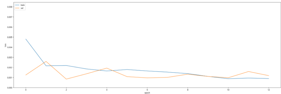
Train Chart
