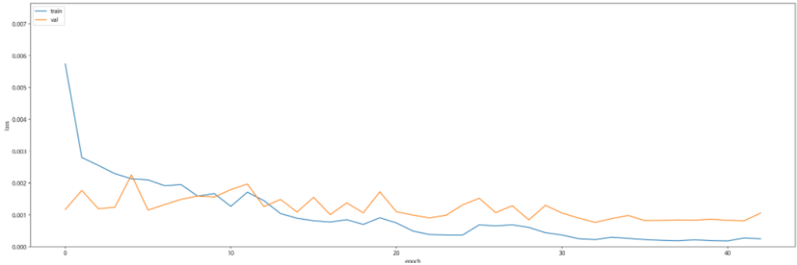
Train Chart
