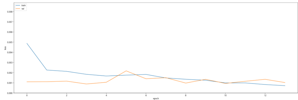
Train Chart
